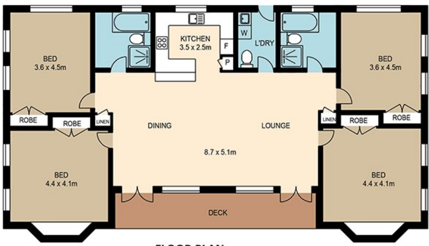
FLOOR PLAN
